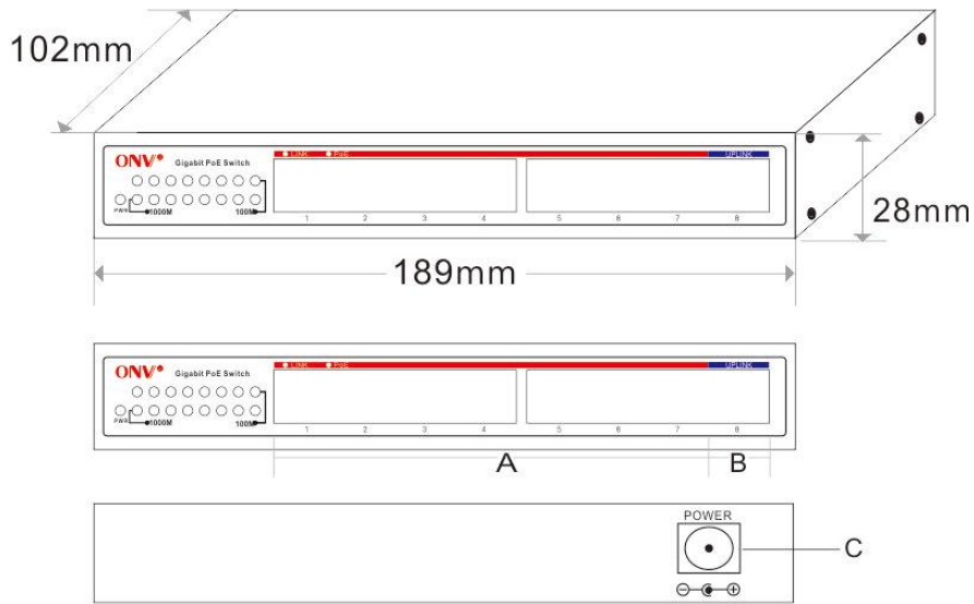
A. 7x Gigabit PoE Ports B. 1x Gigabit Uplink Port C. Power Input Port- DC48-57V
