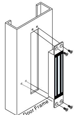
(4) Fix screws
