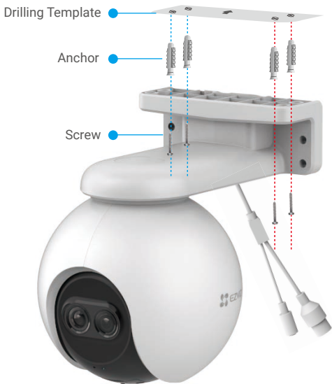
Fig. 1 Ceiling Mount
