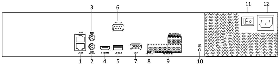
Figure 1-11 iDS-7700NXI-I4/8S Series
