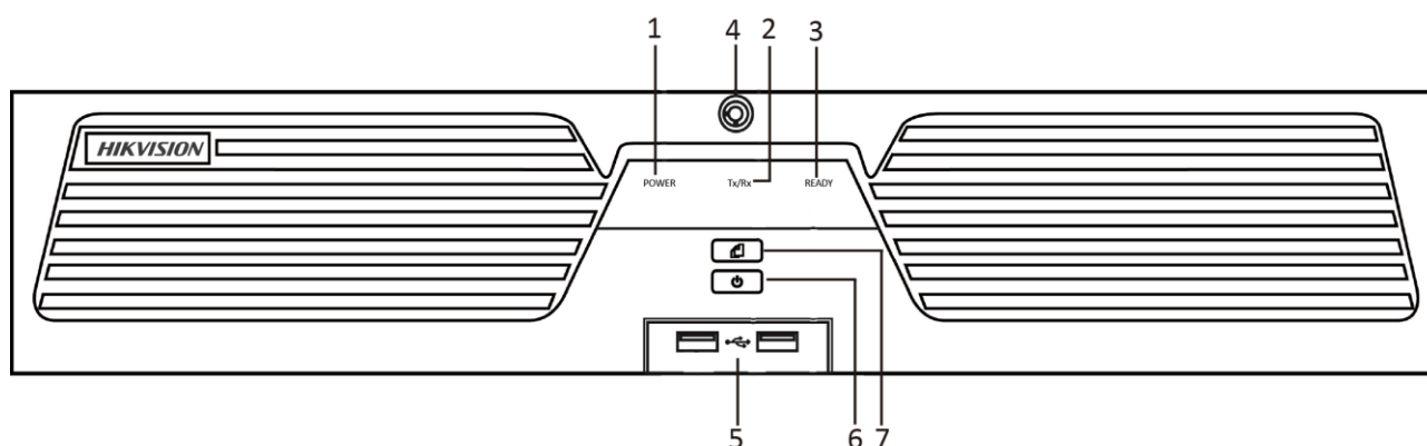
Figure 1-3 Front Panel
