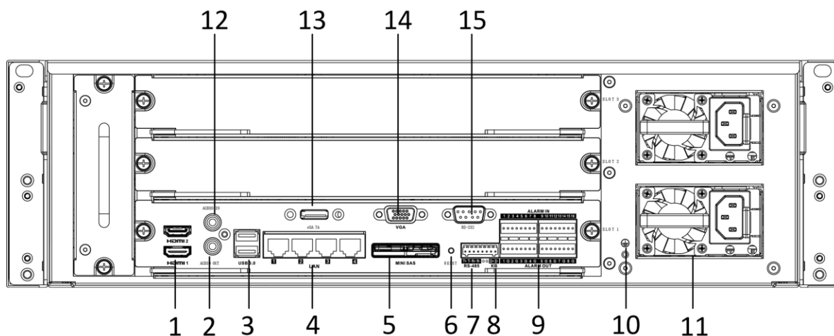
Figure 1-7 Rear Panel
