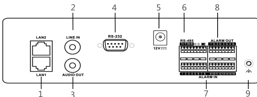
Figure 1-13 Rear Panel
