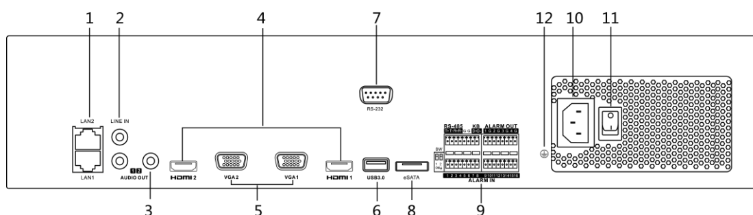
Figure 1-9 Rear Panel
