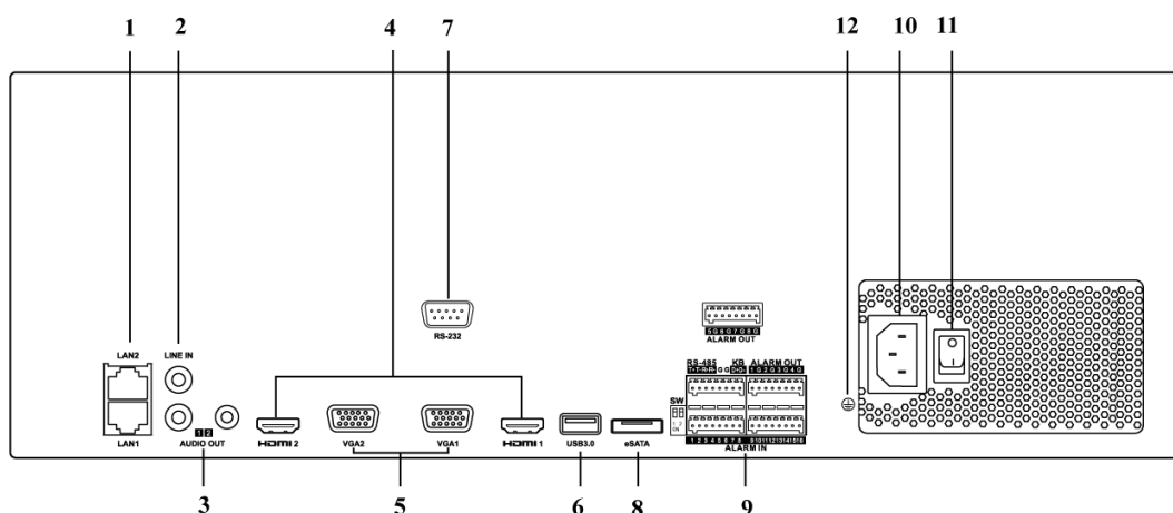
Figure 1-10 Rear Panel
