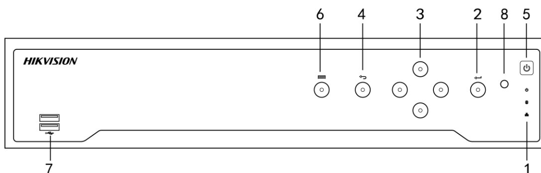
Figure 1-5 Front Panel
