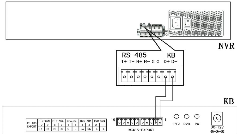
Figure 2-17 Controller Connection
