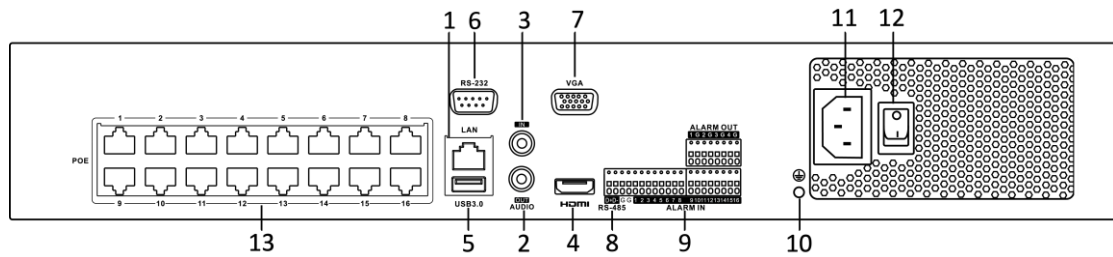
Figure 1-12 iDS-7700NXI-I4/16P/8S Series
