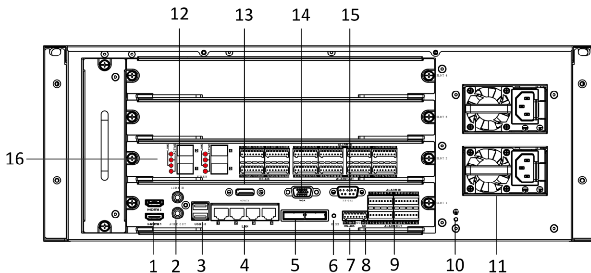
Figure 1-8 iDS-96000NXI-I24 Series
