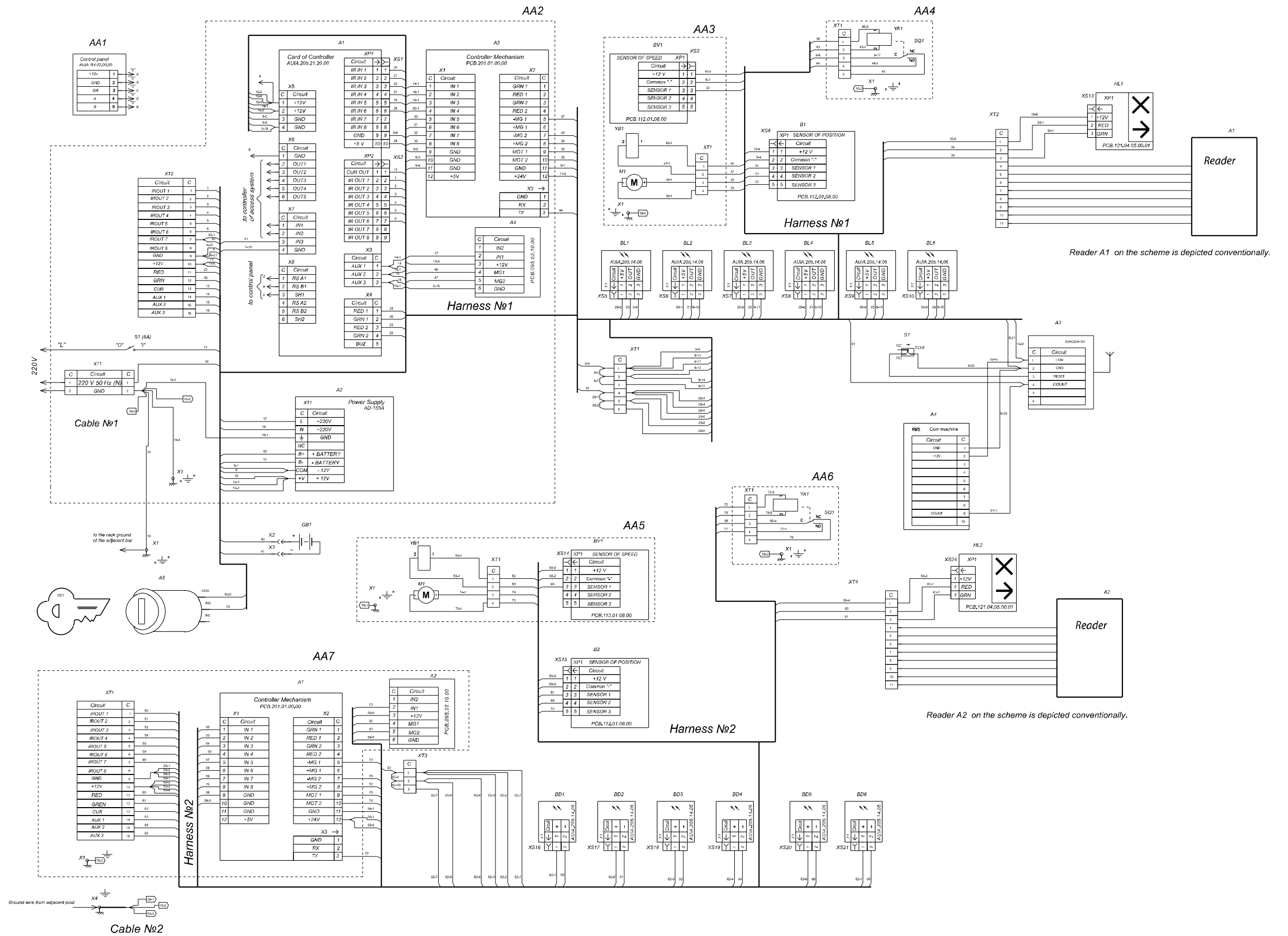
Figure B.2 – Wiring Diagram
