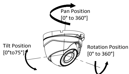
Figure 2-14 3-axis Adjustment
