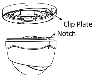
Figure 2-10 Disassemble the Camera
