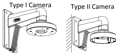
Figure 2-17 Install the Bracket
