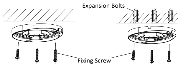
Figure 2-12 Fix the Mounting Base to the Ceiling
