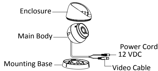
Figure 1-1 Overview of Type I Camera
