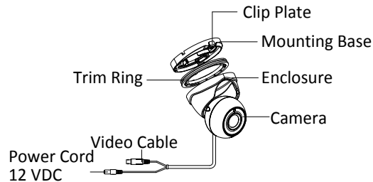
Figure 1-2 Overview of Type II Camera
