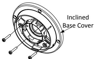
Figure 2-7 Install Turret Camera's Mounting Base
