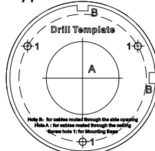
Figure 2-15 Drill Template of the Junction Box
