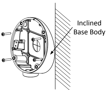
Figure 2-8 Fix the Inclined Base Body
