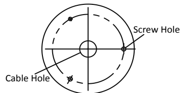
Figure 2-2 Drill Template
