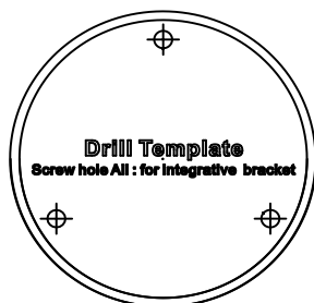
Figure 2-11 Drill Template
