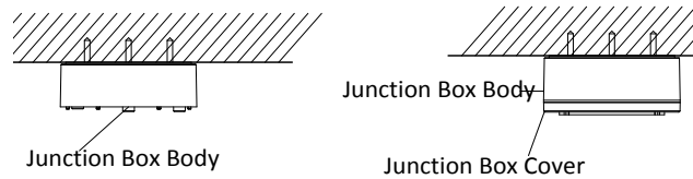
Figure 2-16 Fix the Junction Box
