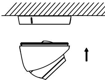
Figure 2-4 Secure the Camera with Mounting Base
