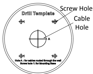
Figure 2-6 The Drill Template
