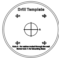
Figure 2-15 Drill Template of the Junction Box
