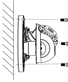
Figure 2-8 Fix the Camera to the Ceiling
