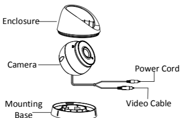
Figure 1. 2 Type II Camera Overview
