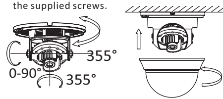
Figure 2-8 3-axis Adjustment & Lower Dome
