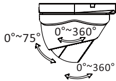
Figure 2-3 3-axis Adjustment
