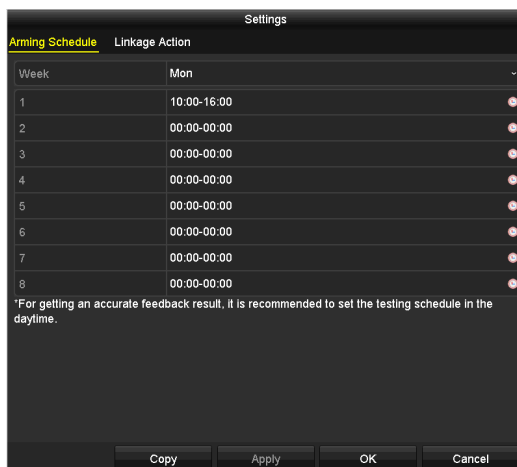
Figure 8-15 Set Arming Schedule of Video Quality Diagnostics
