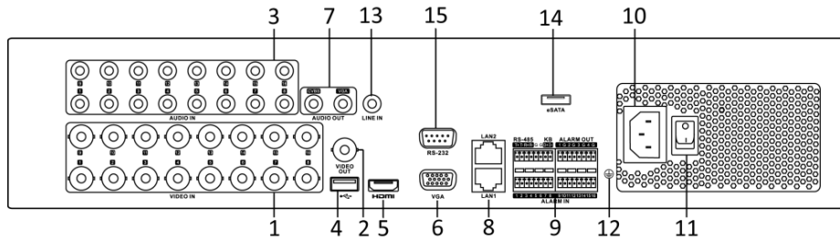
Figure 1-18 Rear Panel of DS-8100HQHI-F8/N
