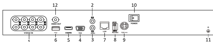
Figure 1-15 Rear Panel of DS-7200HQHI-F2/N
