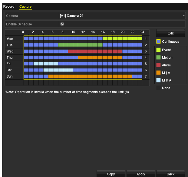
Figure 5-13 Draw the Capture Schedule
