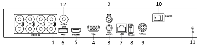
Figure 1-14 Rear Panel of DS-7200HQHI-F1/N
