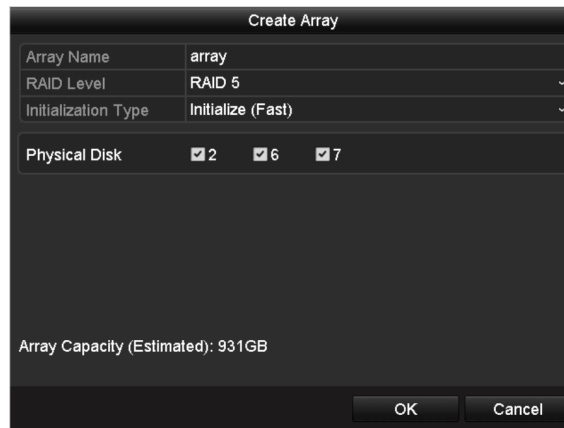
Figure 13-8 Create Array Interface
