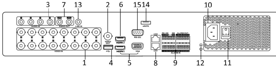
Figure 1-19 Rear Panel of DS-7300HUHI-F4/N
