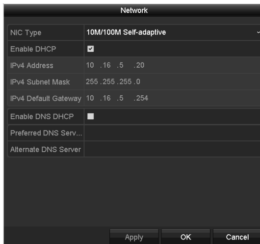
Figure 12-24 Network Parameters Configuration
