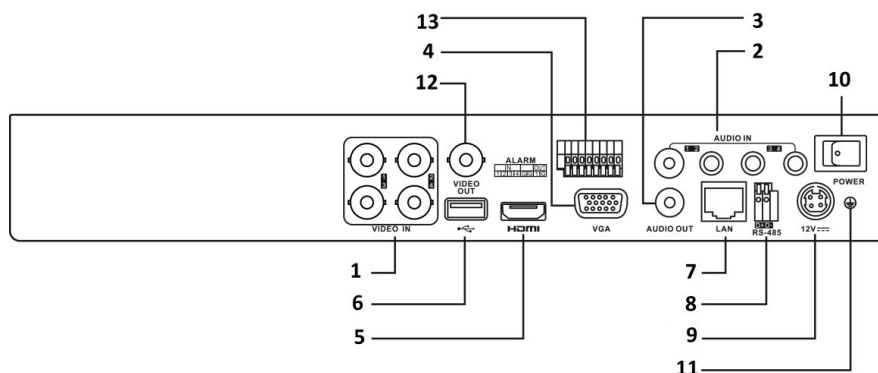
Figure 1-16 Rear Panel of DS-7200HUHI and 7600HUHI-F/N
