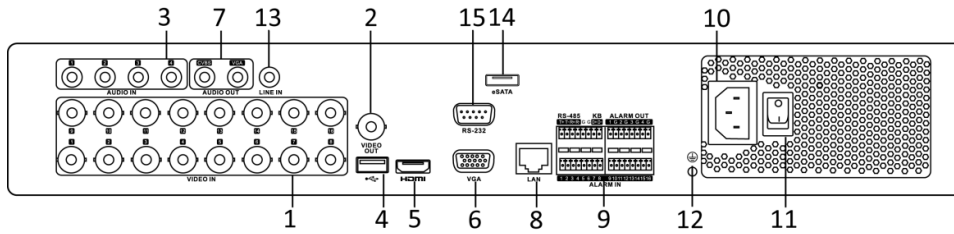
Figure 1-17 Rear Panel of DS-7300HQHI-F4/N
