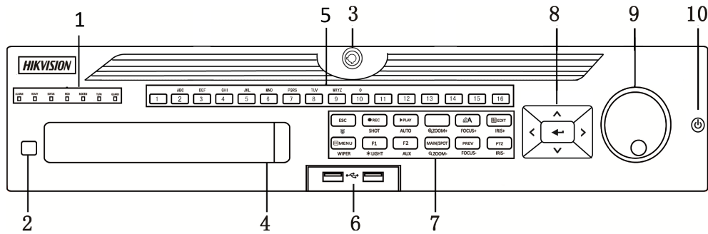
Figure 1-7 Front Panel of DS-9000HUHI-F8/N
