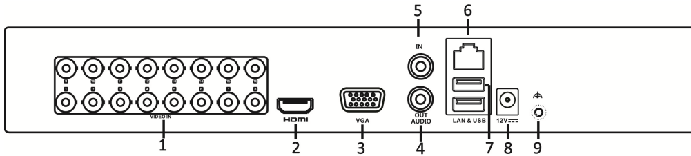
Figure 1-13 Rear Panel of DS-7200HGHI-E
