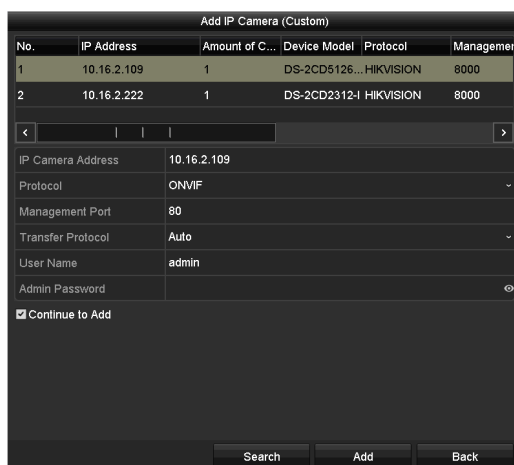
Figure 2-40 Custom Adding IP Camera Interface
