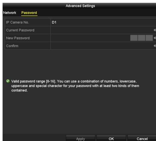
Figure 2-44 Password Configuration of the Camera
