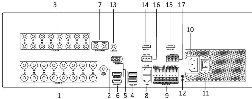
Figure 1-22 Rear Panel of DS-9000HUHI-F16/N
