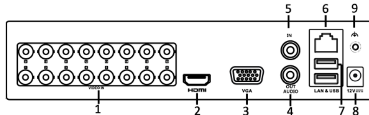
Figure 1-12 Rear Panel of DS-7200HGH-F (/N)
