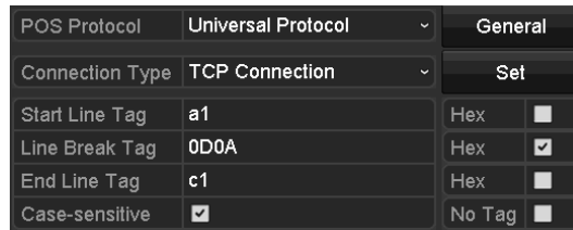
Figure 9-3 Universal Protocol Settings
