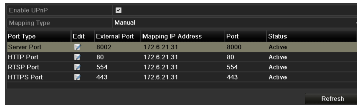
Figure 12-11 UPNP™ Settings Finished-Manual
