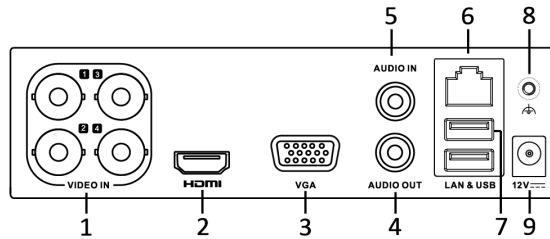
Figure 1-11 Rear Panel of DS-7100
