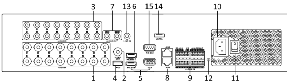
Figure 1-21 Rear Panel of DS-9000HUHI-F8/N
