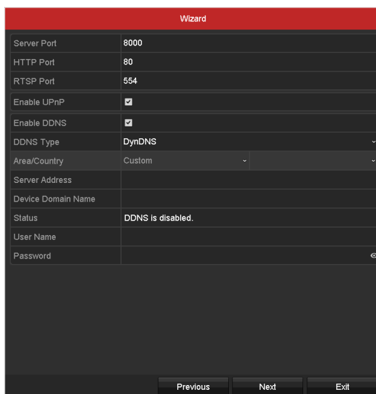
Figure 2-22 Set Advanced Network Parameters
