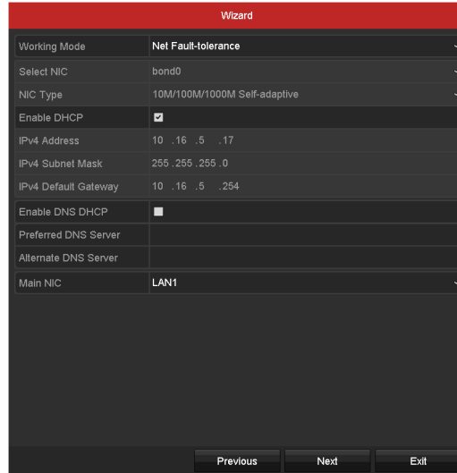
Figure 2-20 General Network Configuration
