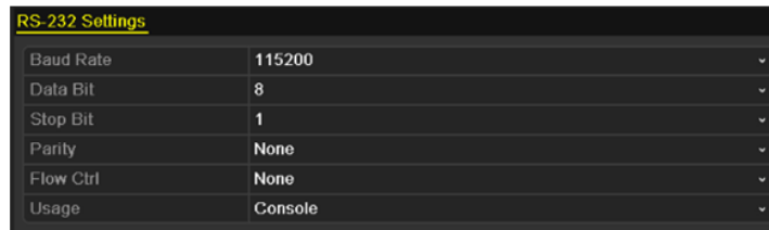
Figure 17-4 RS-232 Settings Interface
