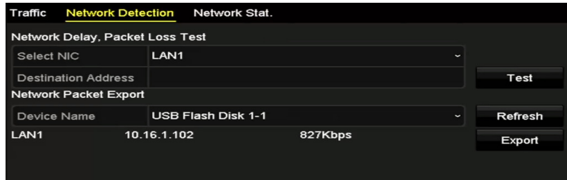
Figure 12-19 Network Detection Interface
