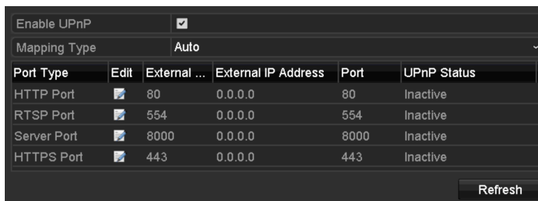
Figure 12-8 UPnP™ Settings Interface
