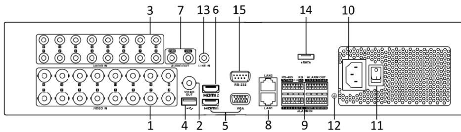
Figure 1-20 Rear Panel of DS-8100HUHI-F8/N
