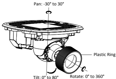
Figure 2-8 3-Axis Adjustment
