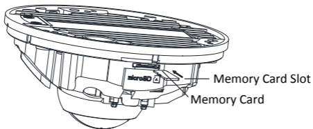
Figure 2-11 Install the Memory Card
