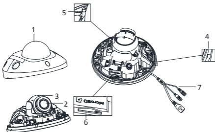
Figure 1-2 Overview of Type II Mobile Network Mini Dome Camera
