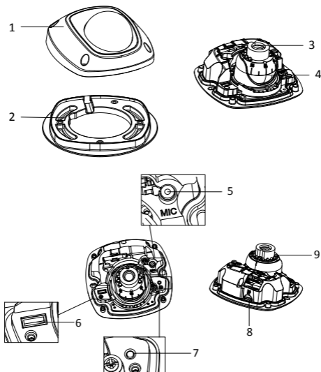
Figure 1-1 Overview of Type I Mobile Network Mini Dome Camera
