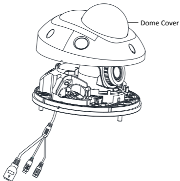
Figure 2-10 Disassemble the Camera
