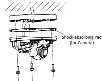
Figure 2-14 Secure Camera Body
