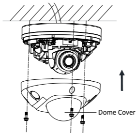
Figure 2-16 Install the Dome Cover
