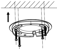
Figure 2-6 Install the Mounting Base
