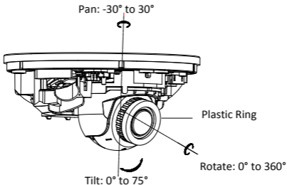
Figure 2-15 3-Axis Adjustment
