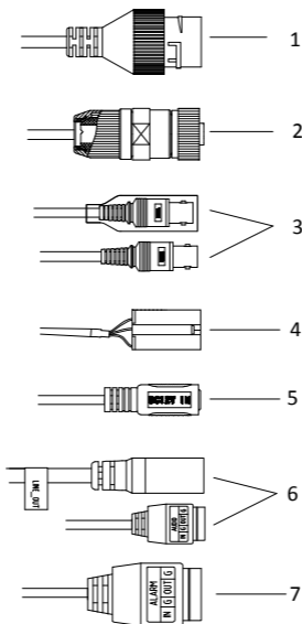
Figure 1-3 Cable Overview
