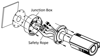
Figure 2-14 Mounting with a Junction Box
