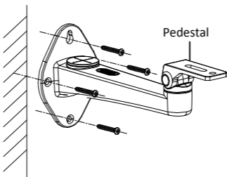
Figure 2-5 Install the Wall Mounting Bracket
