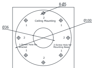
Figure 2-11 Drilling Holes in the Wall/Ceiling
