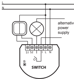
Fig.1 Circuit diagrams for Fibaro Switch.
